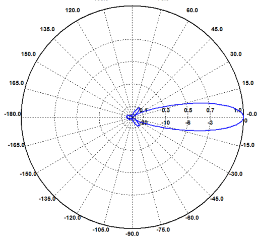
H-Ebene / H-Plane 6.0 GHz
