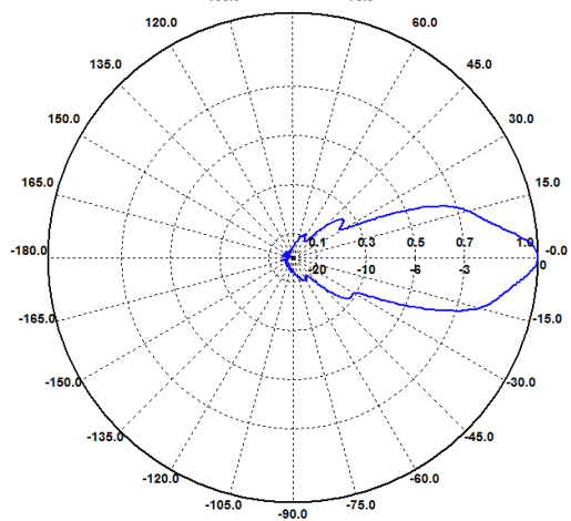
E-Ebene / E-Plane 6.0 GHz
